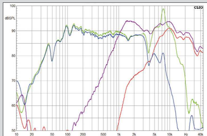
The woofer shows cone resonances at 7.5 kHz, which are well-filtered by the crossover. The tweeter could also be used at lower frequencies
