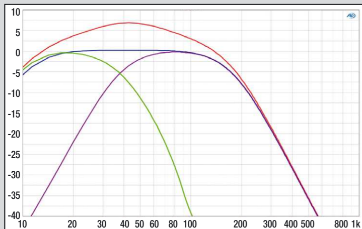
The X-2000.1 pleases with cleanly working filters, also the subsonic scores with a steep 24 dB/oct. slope
