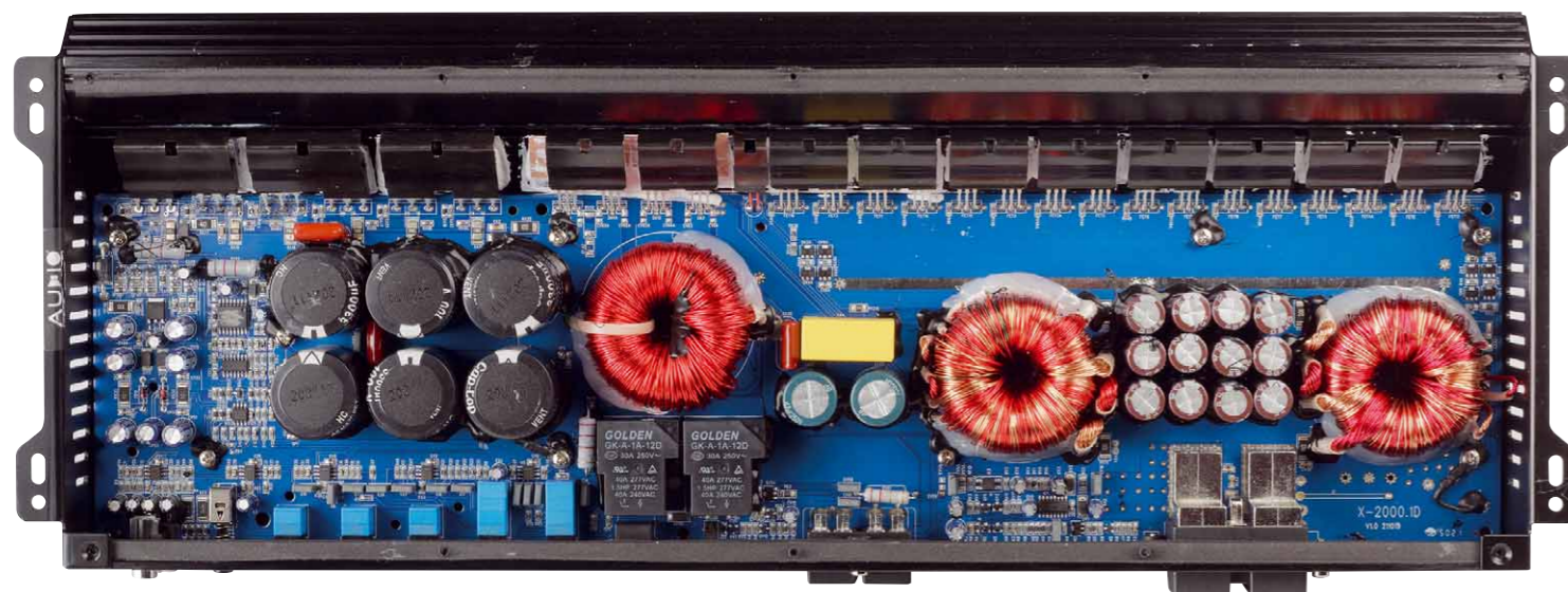
22 high power MOSFETs team on the heatsink. The transformers and the filter coil are gigantic
