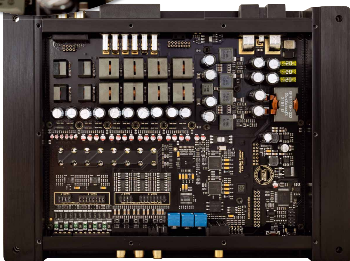
Everything on the board is new. A highlight is the DSP department, which now has two processor chips
