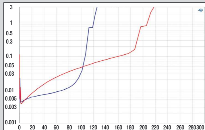
The ZXS700/4 operates with very low distortion, especially at 4 ohms. With 120 and 210 Watts, there is also plenty of power for small loudspeakers
