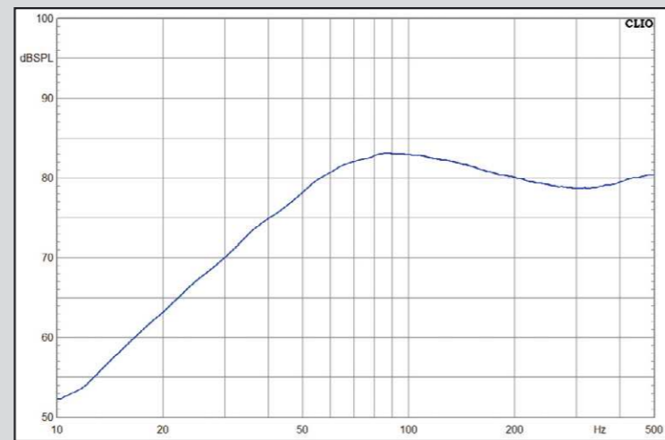
The VXP84 shows the flat decay towards low frequencies typical for closed subwoofers. You hear much deeper bass than the diagram suggests
