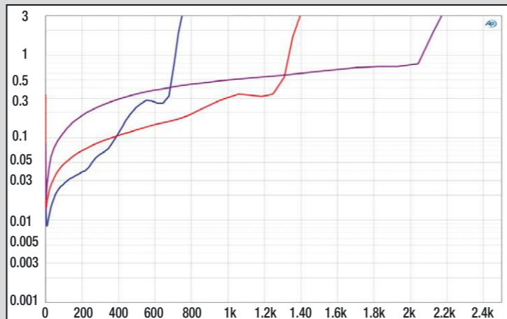
The X-2000.1 D can produce up to over 2000 watts into 1 ohm. However, the lower the load, the more distortion it produces
