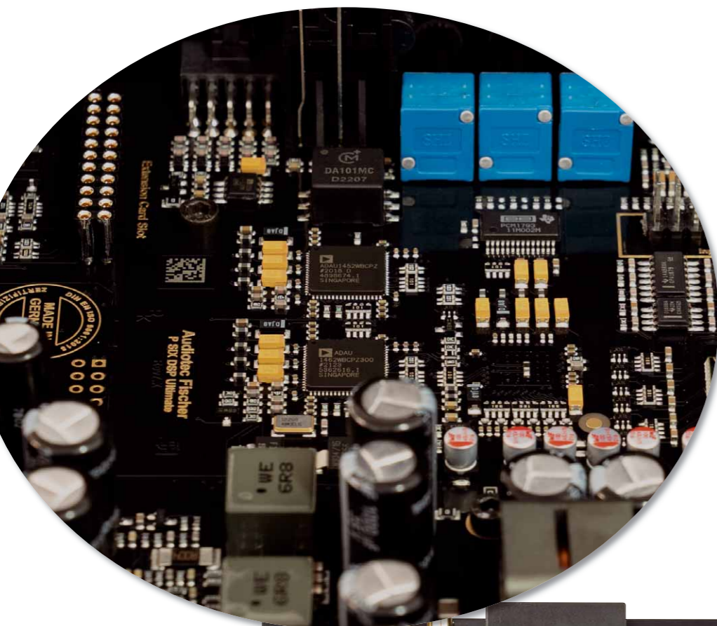
Everything on the board is new. A highlight is the DSP department, which now has two processor chips
