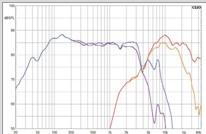
The woofer and tweeter run smoothly both on-axis and under an angle
