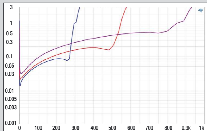
Power burst with the ZXS900/1: With moderate distortion, there are 300, 550, and at the kink, almost 900 watts for the sub
