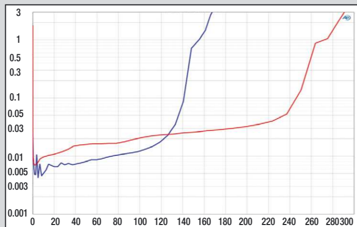
As the smallest of the series, the ZXS550/2 manages nearly 160 and 280 watts per channel with minimal distortion. A terrific performance!
